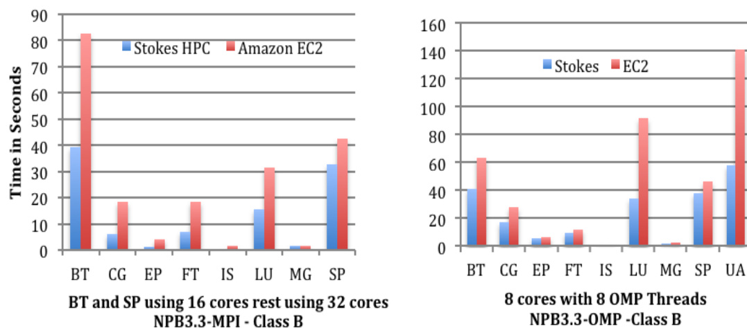
Figure 5: NPB MPI and OMP Benchmark Results 37
